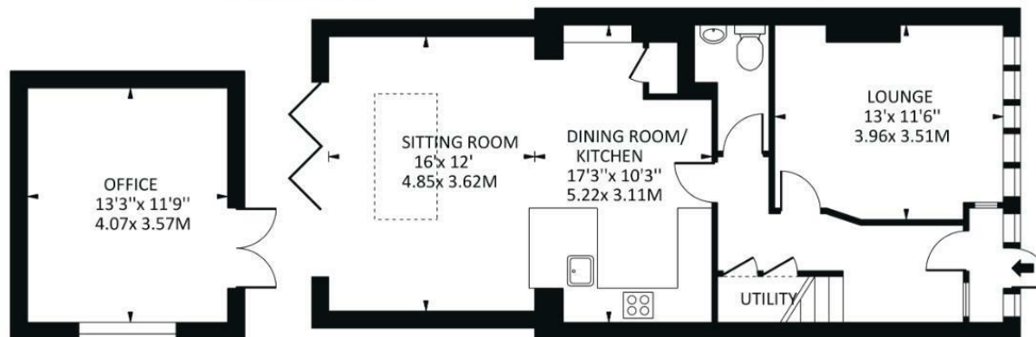
GROUND FLOOR
